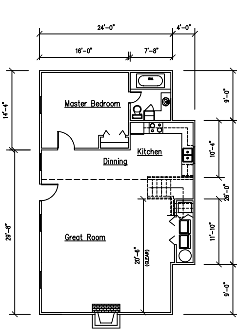
GROUND LEVEL
